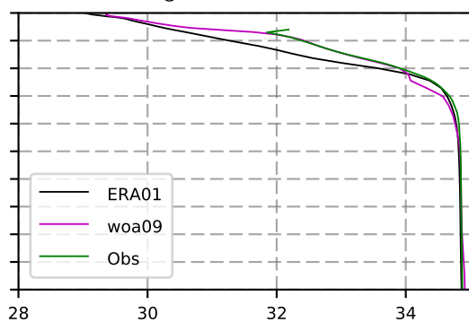
2011 mean Salinity @ moor Arctic B box
