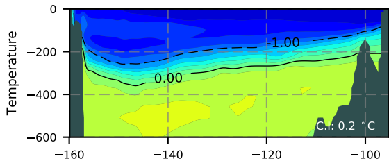
ERA01 / Beaufort Section 1982
