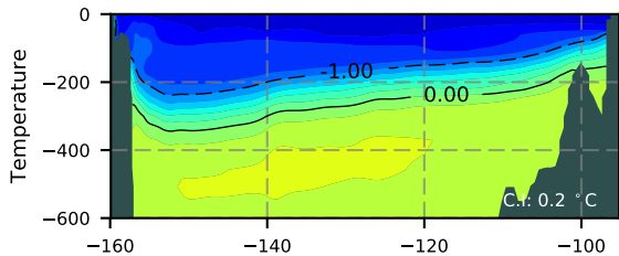
ERA01 / Beaufort Section 1988
