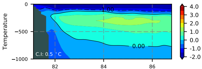
ERA01 / Kara Section 1980
