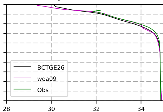
1962 mean Salinity @ moor Arctic B box
