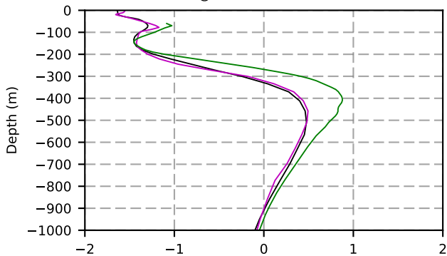
1962 mean temperature @ moor Arctic B box
