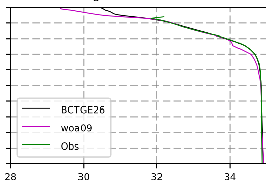
1967 mean Salinity @ moor Arctic B box
