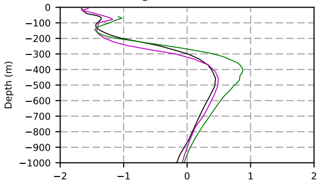
1967 mean temperature @ moor Arctic B box
