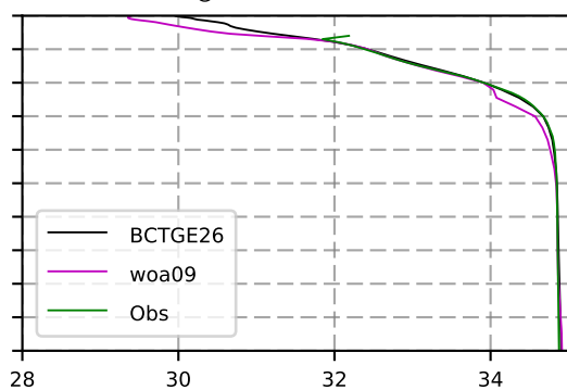
1968 mean Salinity @ moor Arctic B box
