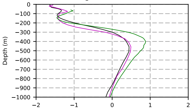
1968 mean temperature @ moor Arctic B box
