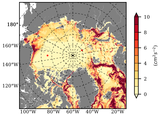
BVHGE24 mean EKE @ 0 m over 1959
