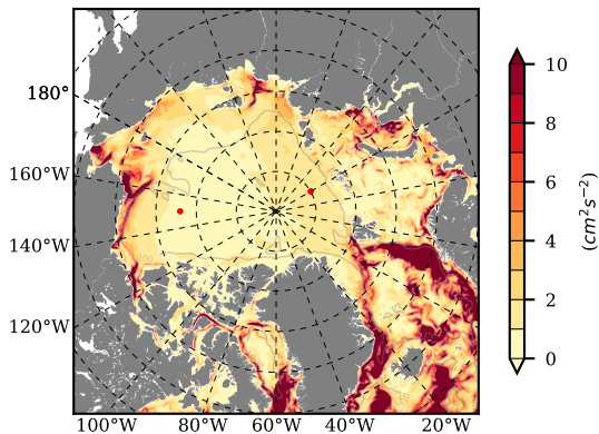
BVHGE24 mean EKE @ 0 m over 1961
