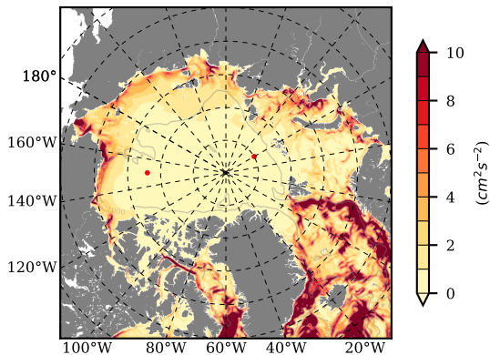
BVHGE24 mean EKE @ 0 m over 1965
