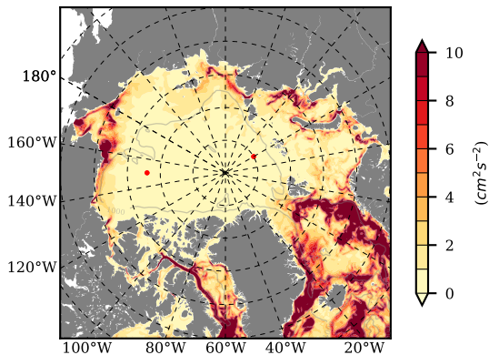
BVHGE24 mean EKE @ 0 m over 1967
