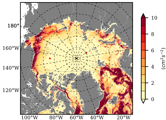
BVHGE24 mean EKE @ 0 m over 1968
