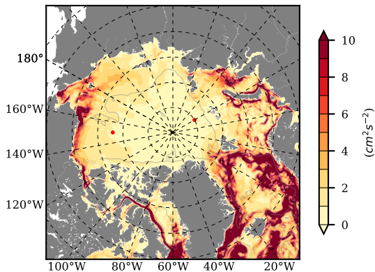
BVHGE24 mean EKE @ 0 m over 1969
