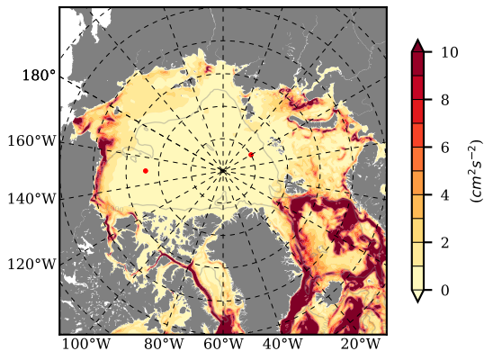
BVHGE24 mean EKE @ 0 m over 1970
