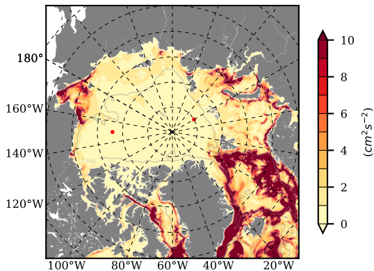
BVHGE24 mean EKE @ 0 m over 1972
