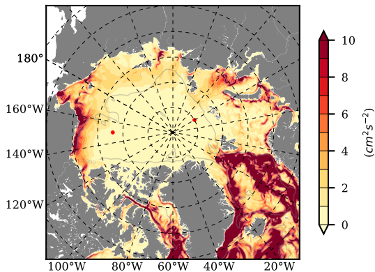
BVHGE24 mean EKE @ 0 m over 1974
