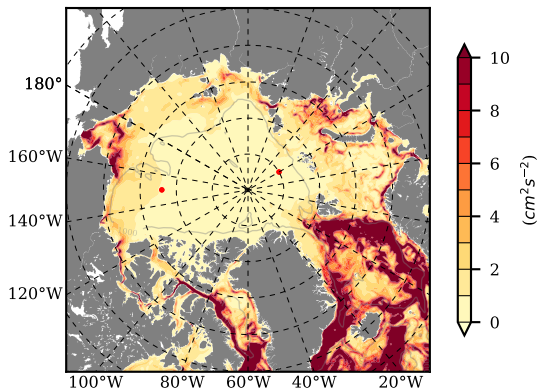
BVHGE24 mean EKE @ 0 m over 1976
