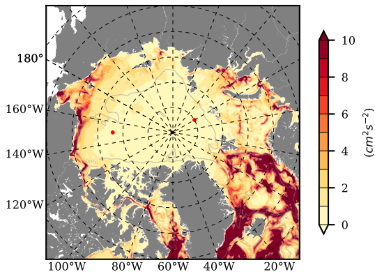
BVHGE24 mean EKE @ 0 m over 1977
