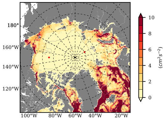
BVHGE24 mean EKE @ 0 m over 1978
