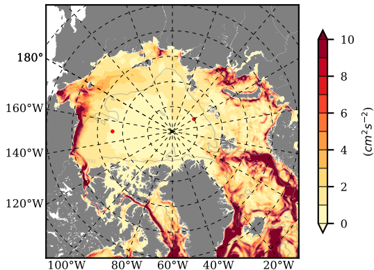
BVHGE24 mean EKE @ 0 m over 1980
