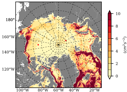
BVHGE24 mean EKE @ 0 m over 1981
