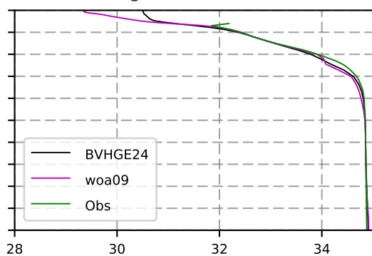
1964 mean Salinity @ moor Arctic B box
