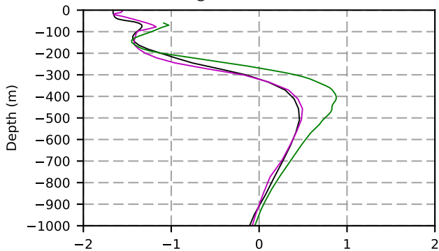
1964 mean temperature @ moor Arctic B box
