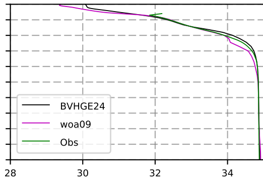
1969 mean Salinity @ moor Arctic B box
