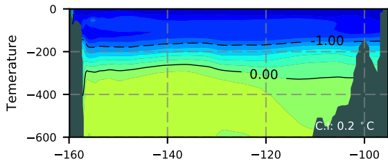
BVHGE24 / Beaufort Section 1982
