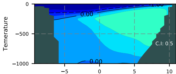
BVHGE24 / FramS Section 1981
