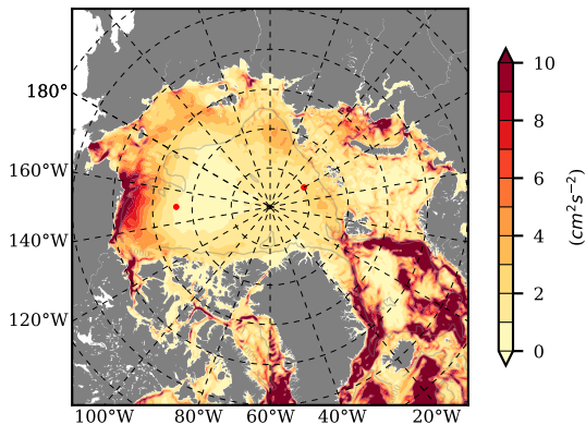
BVHGE25 mean EKE @ 0 m over 1960
