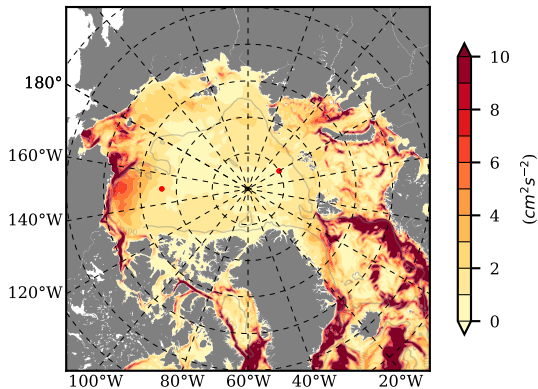
BVHGE25 mean EKE @ 0 m over 1962
