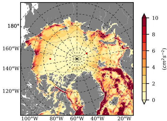
BVHGE25 mean EKE @ 0 m over 1964
