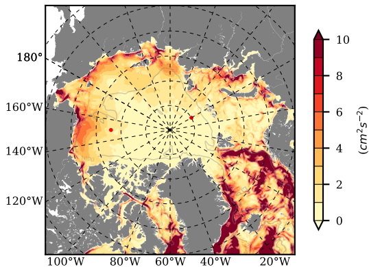
BVHGE25 mean EKE @ 0 m over 1965
