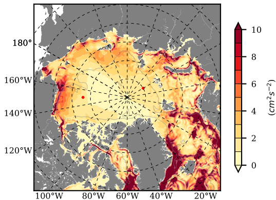
BVHGE25 mean EKE @ 0 m over 1966
