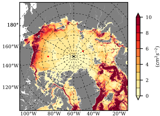
BVHGE25 mean EKE @ 0 m over 1968
