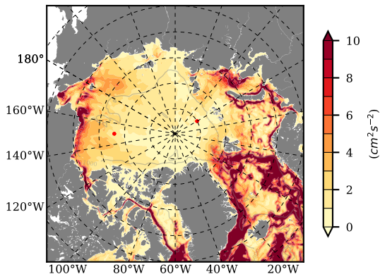
BVHGE25 mean EKE @ 0 m over 1969
