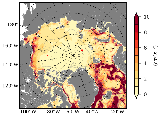
BVHGE25 mean EKE @ 0 m over 1970
