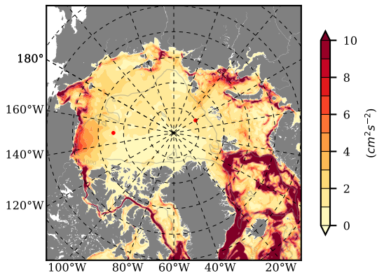
BVHGE25 mean EKE @ 0 m over 1971
