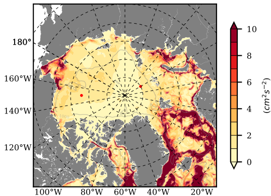
BVHGE25 mean EKE @ 0 m over 1972
