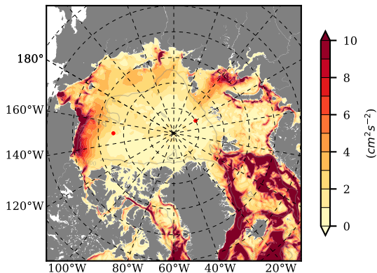
BVHGE25 mean EKE @ 0 m over 1974
