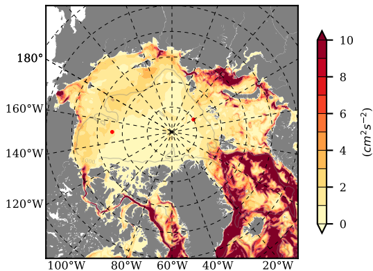
BVHGE25 mean EKE @ 0 m over 1975
