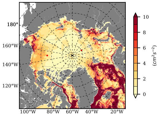
BVHGE25 mean EKE @ 0 m over 1976
