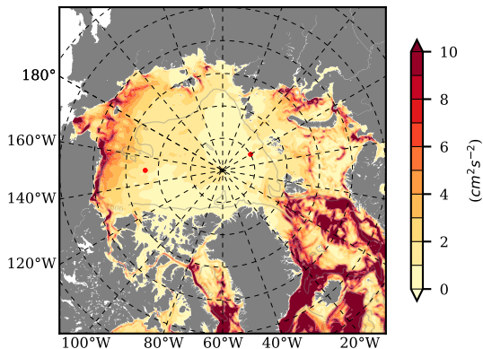
BVHGE25 mean EKE @ 0 m over 1977
