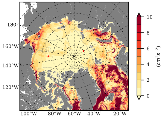
BVHGE25 mean EKE @ 0 m over 1978
