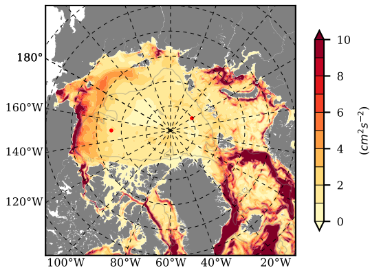
BVHGE25 mean EKE @ 0 m over 1980
