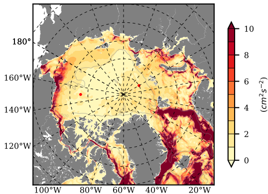
BVHGE25 mean EKE @ 0 m over 1982
