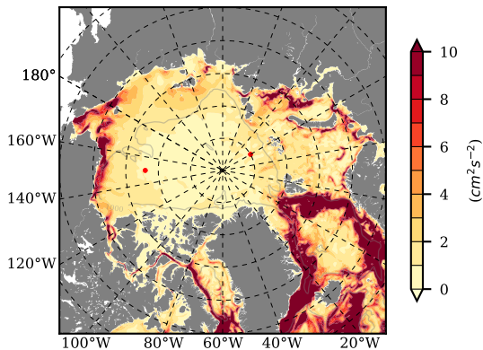
BVHGE25 mean EKE @ 0 m over 1983
