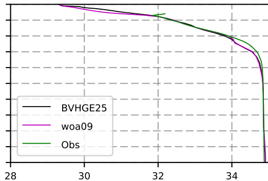
1960 mean Salinity @ moor Arctic B box
