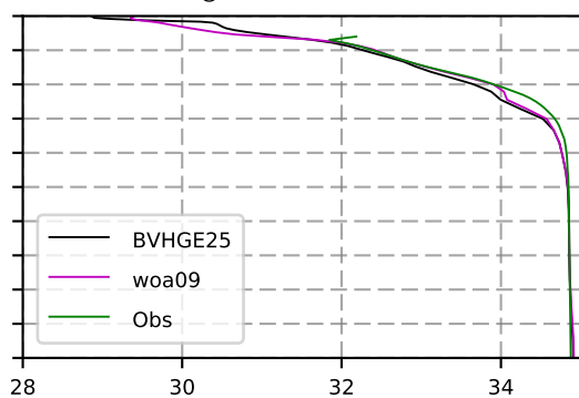
1961 mean Salinity @ moor Arctic B box
