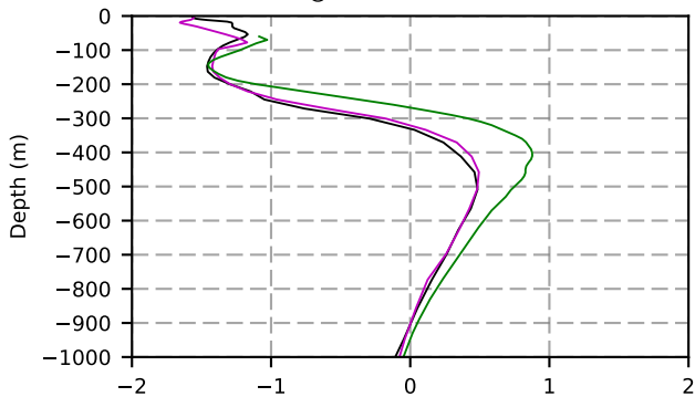
1961 mean temperature @ moor Arctic B box
