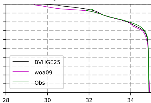
1965 mean Salinity @ moor Arctic B box
