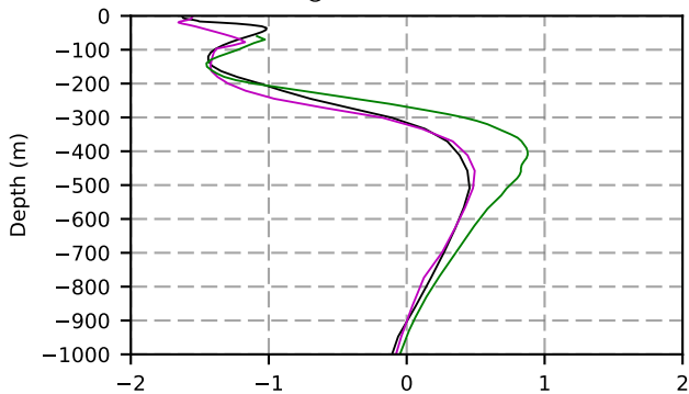
1965 mean temperature @ moor Arctic B box
