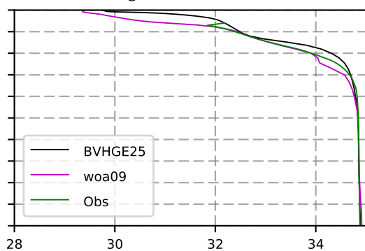
1972 mean Salinity @ moor Arctic B box
