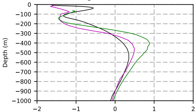
1972 mean temperature @ moor Arctic B box
