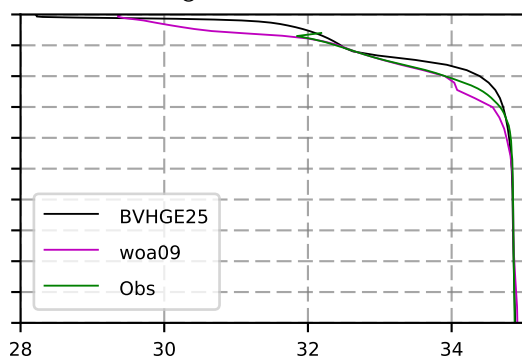
1974 mean Salinity @ moor Arctic B box
