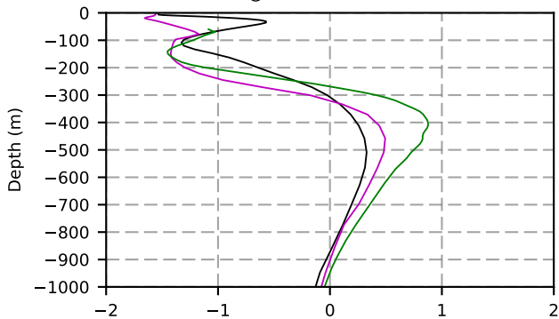
1974 mean temperature @ moor Arctic B box
