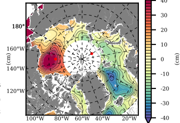
Mean DOT from Armitage et al. 2017 2010
