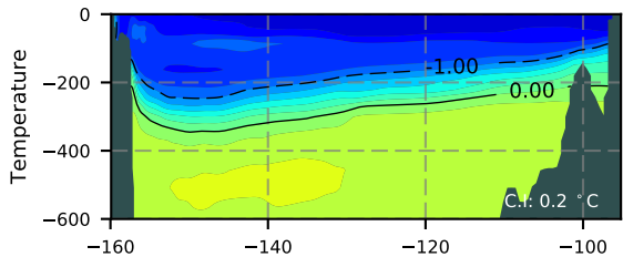
BCTTWINERA5 / Beaufort Section 1995
